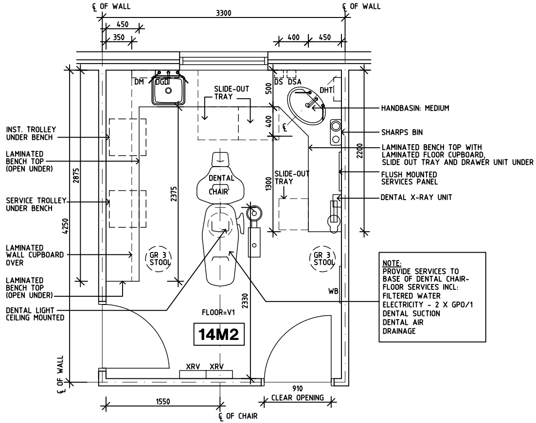
PLAN
