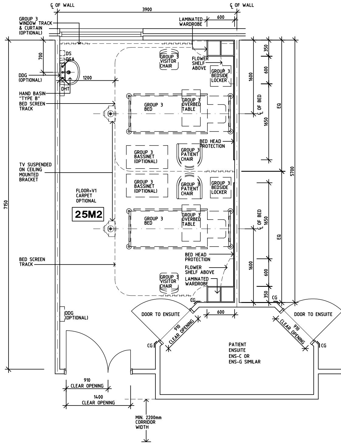
PLAN
