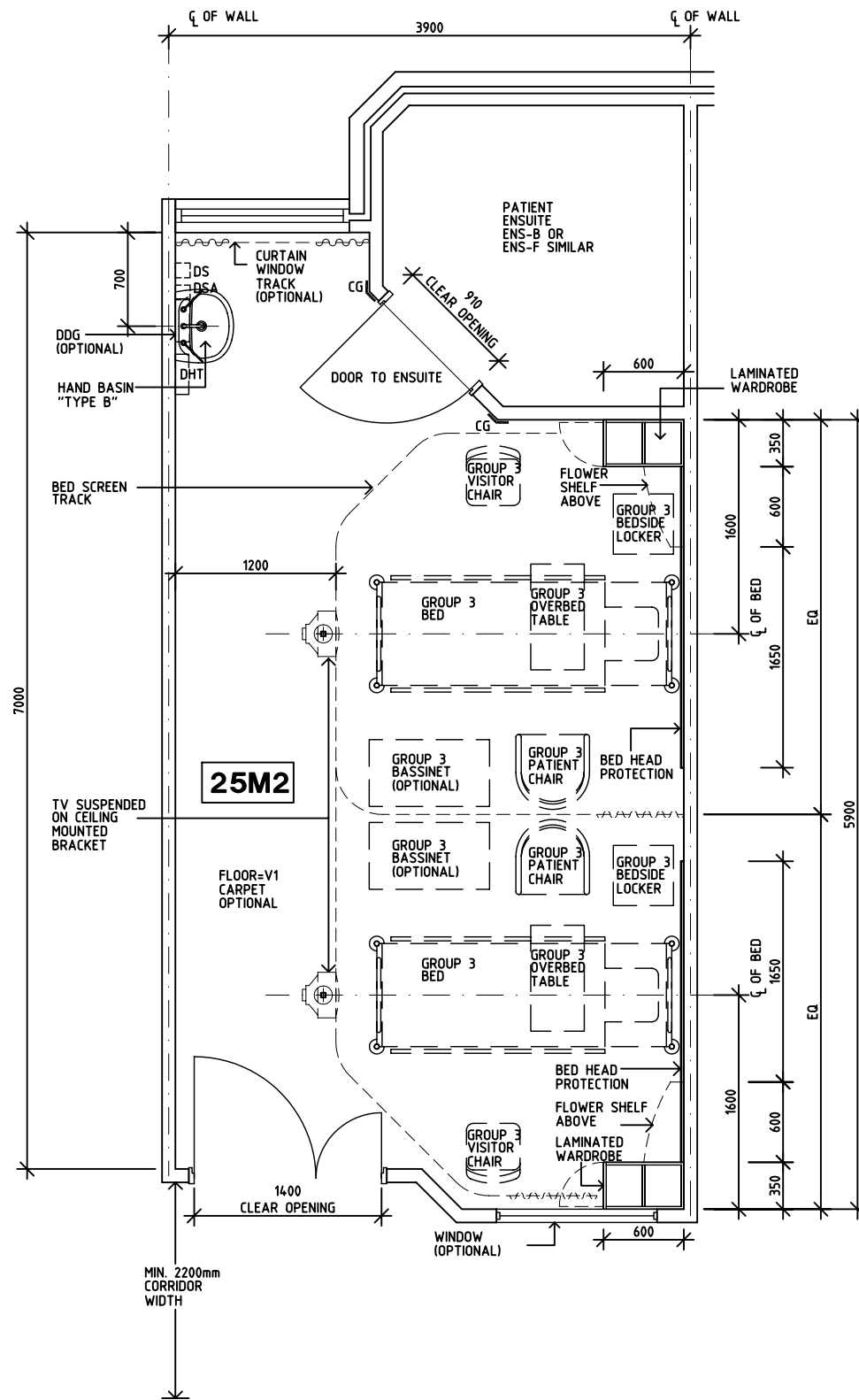
PLAN
