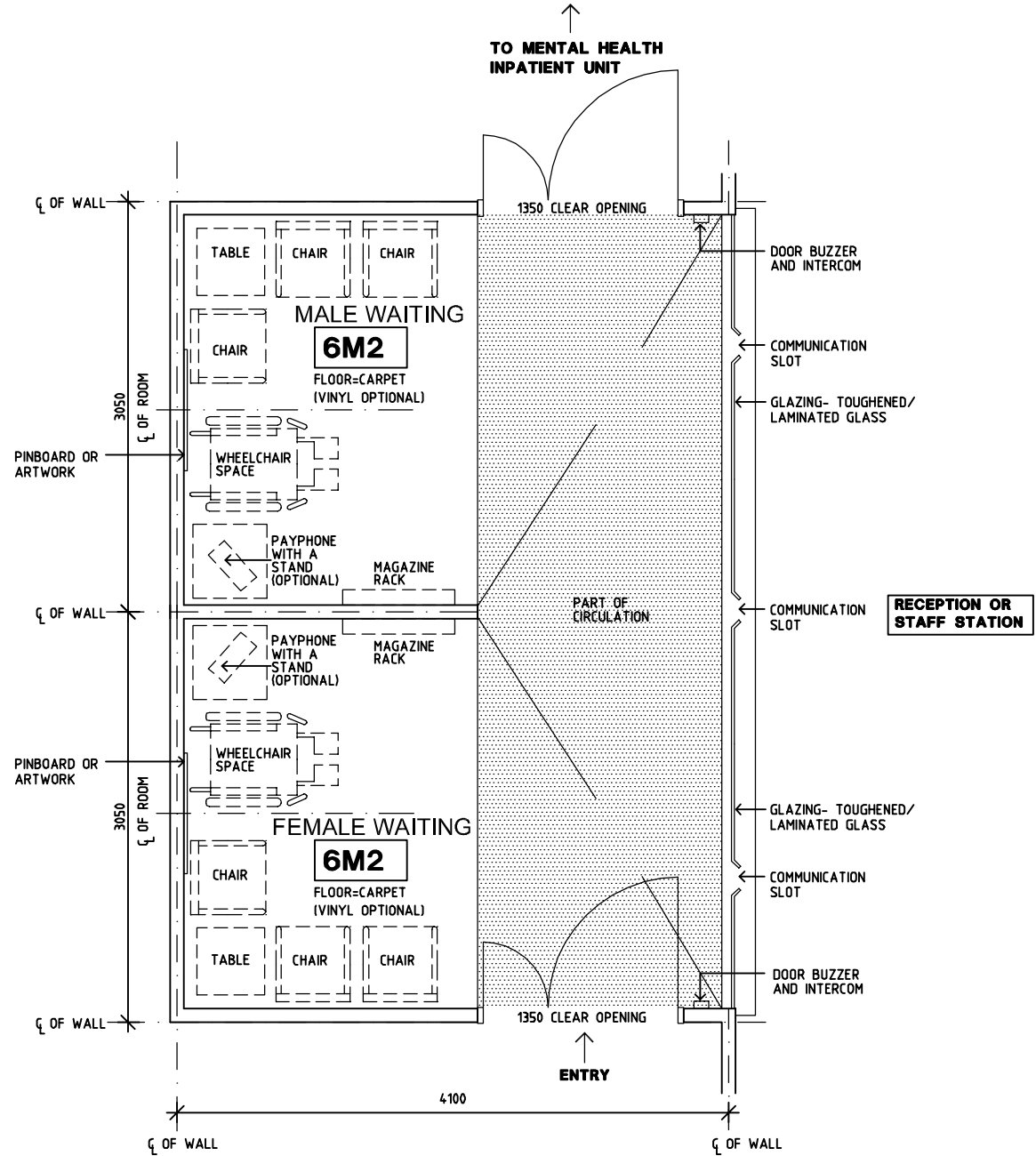
PLAN
