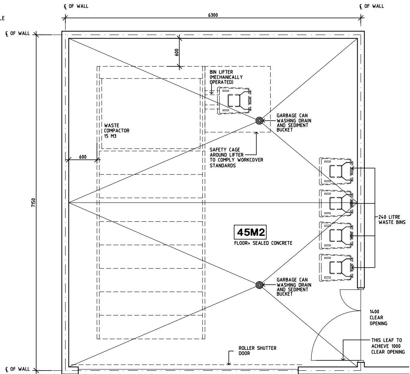
PLAN
