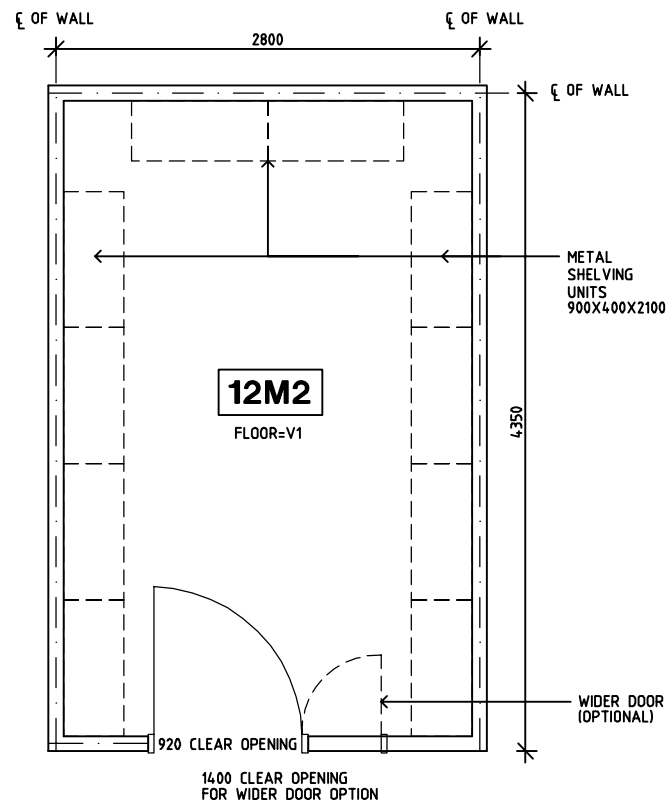
PLAN
