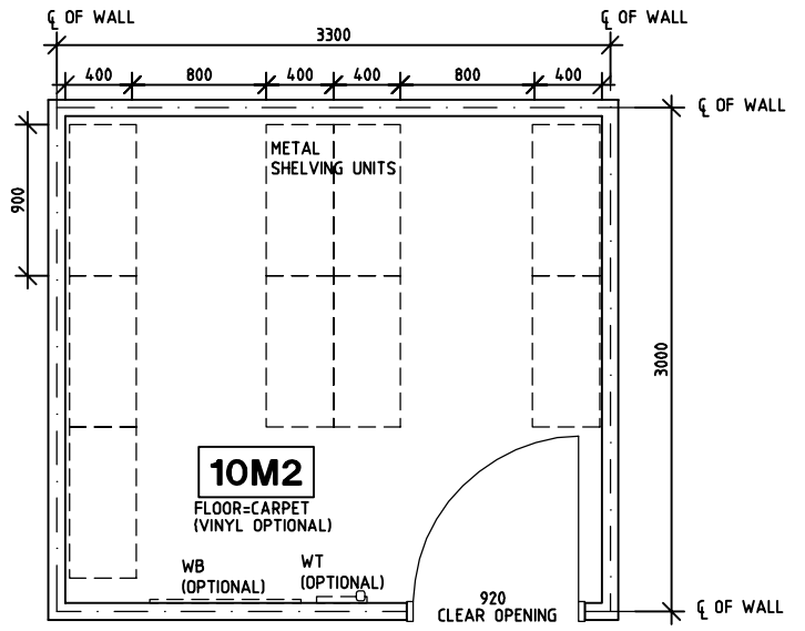
OPTION 2- static shelving PLAN
