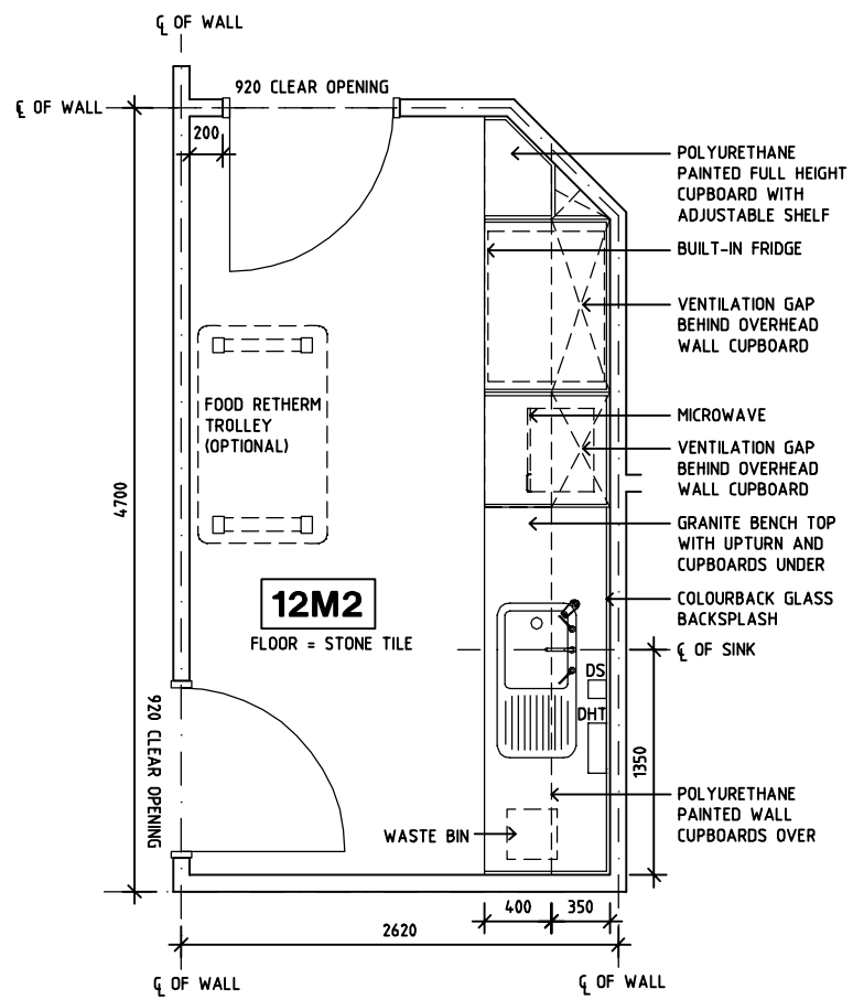
PLAN
