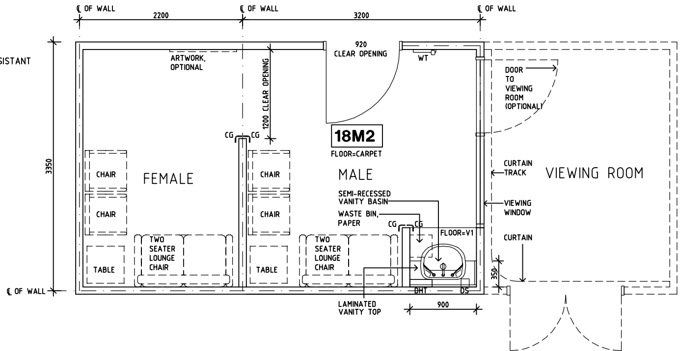
PLAN
