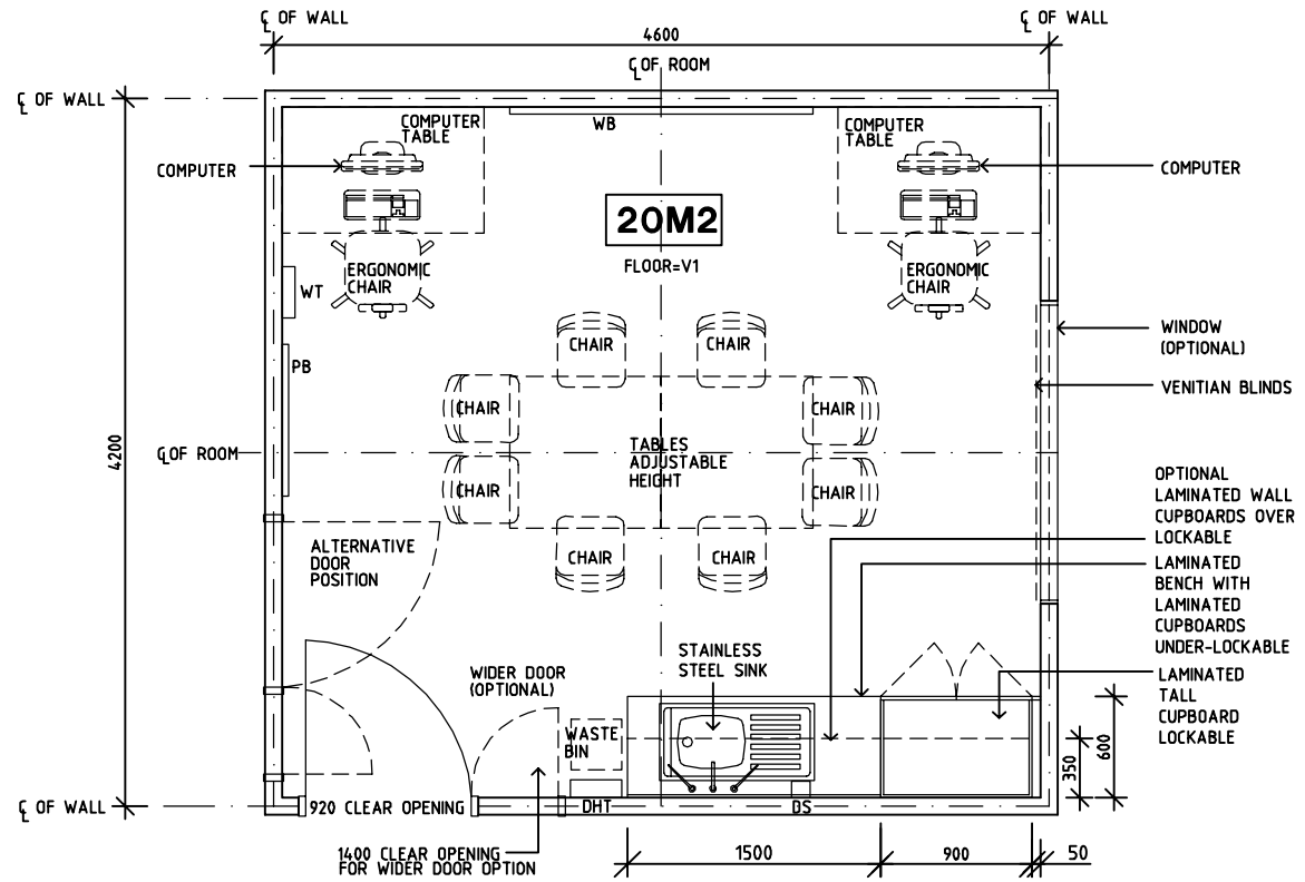
PLAN
