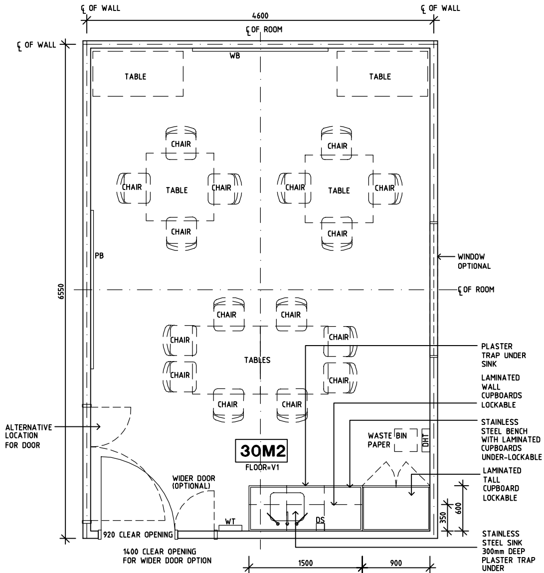
PLAN
