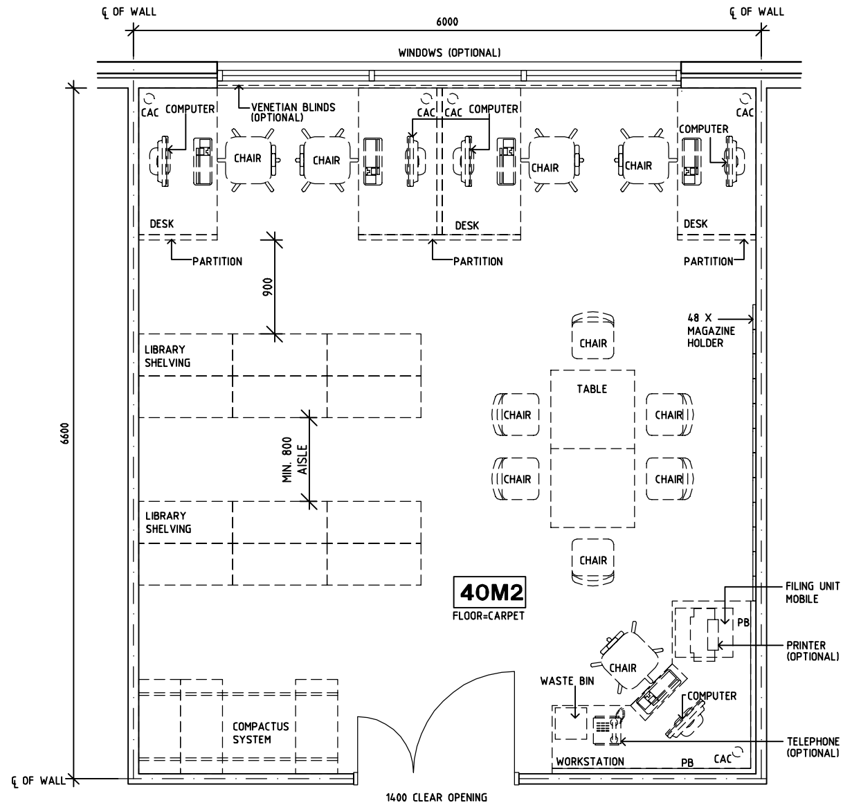
PLAN
