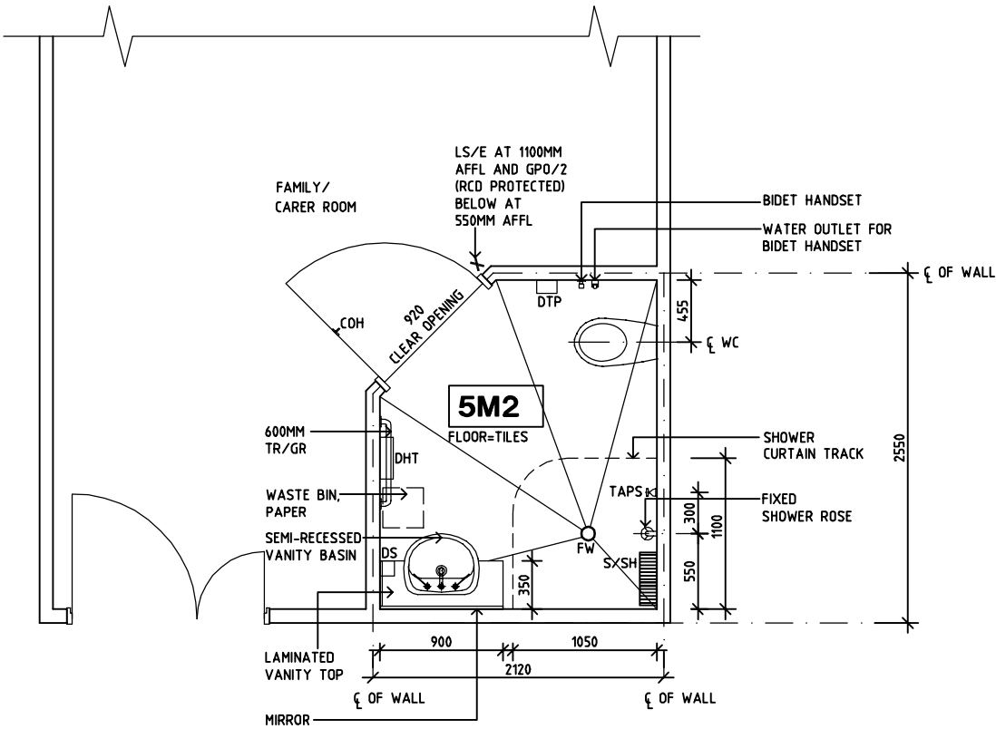
PLAN
