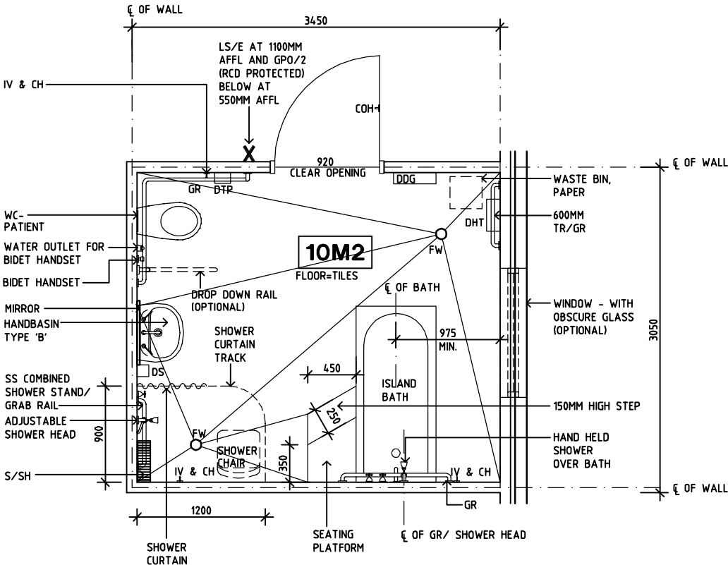
PLAN
