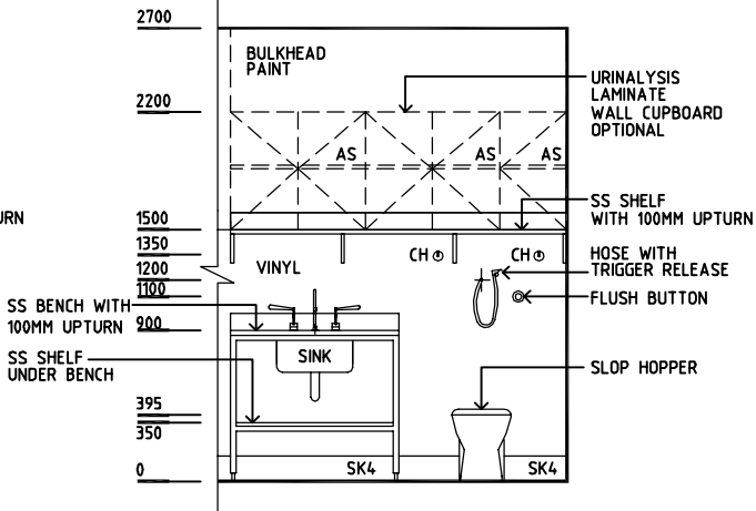
ELEVATION 2 ALTERNATIVE
