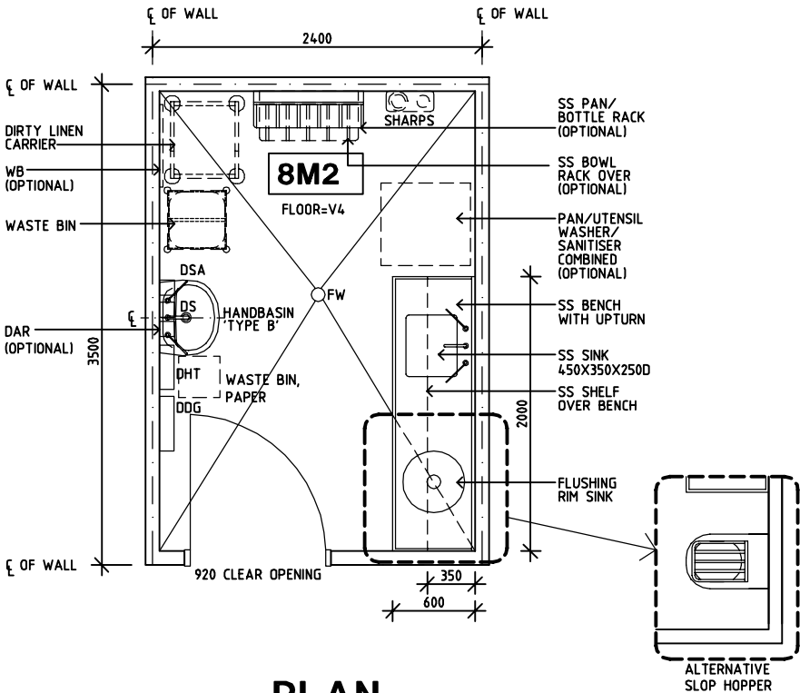
PLAN
