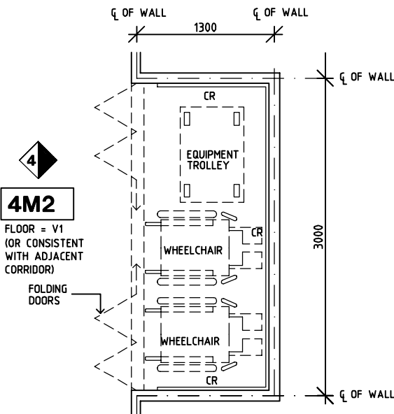
PLAN
