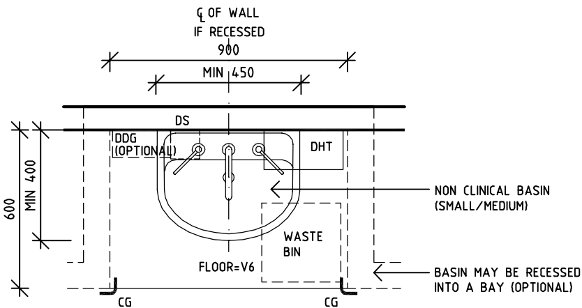
TYPE C - NON CLINICAL BASIN (SMALL/MEDIUM) OPTION 1 PLAN
