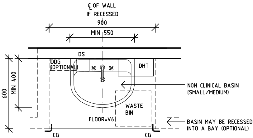
TYPE C - NON CLINICAL BASIN (SMALL/MEDIUM) OPTION 3 PLAN
