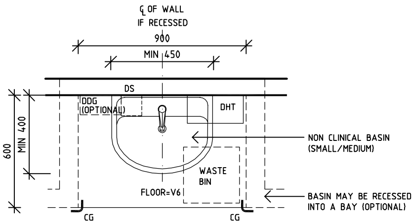
TYPE C - NON CLINICAL BASIN (SMALL/MEDIUM) OPTION 2 PLAN
