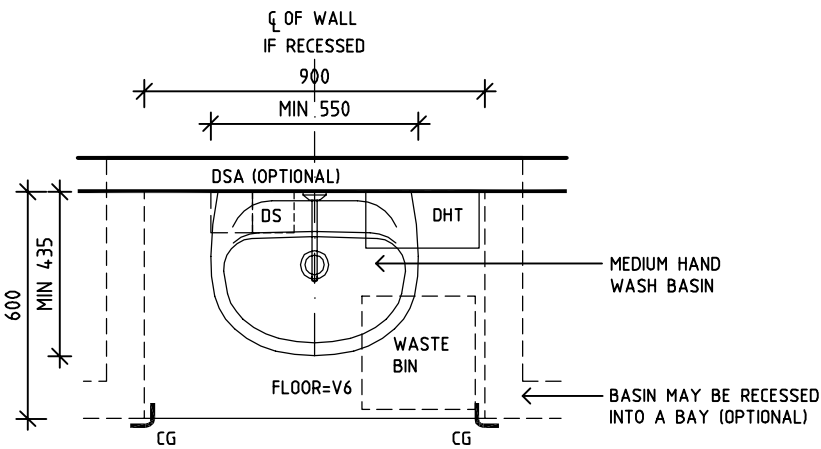
BASIN (MEDIUM) - OPTION 4 PLAN
