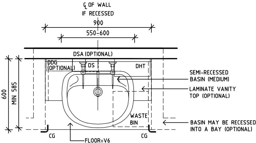
BASIN (MEDIUM) SEMI RECESSED - OPTION 3 PLAN
