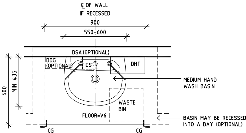
TYPE B - CLINICAL BASIN (MEDIUM) OPTION 1 PLAN
