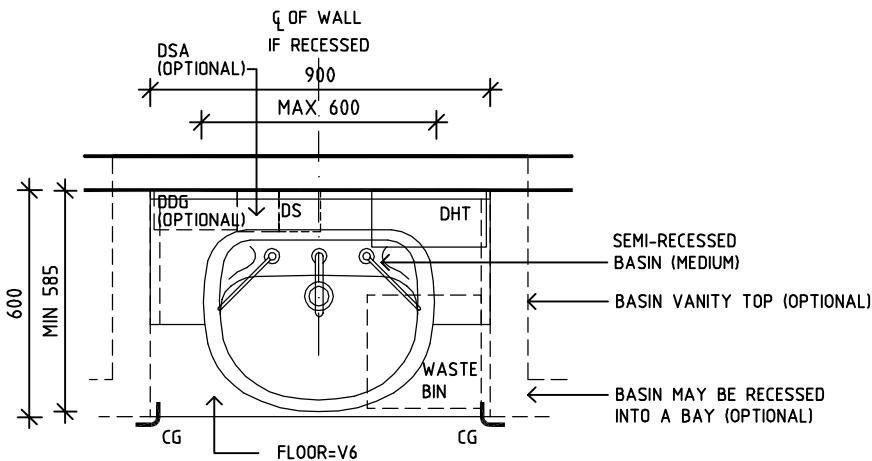
BASIN (MEDIUM) SEMI RECESSED - OPTION 2 PLAN
