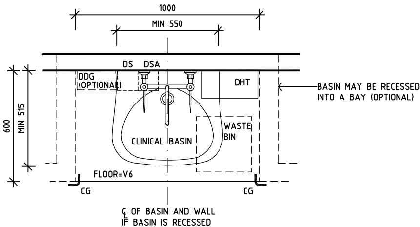
TYPE A - CLINICAL BASIN (LARGE) PLAN
