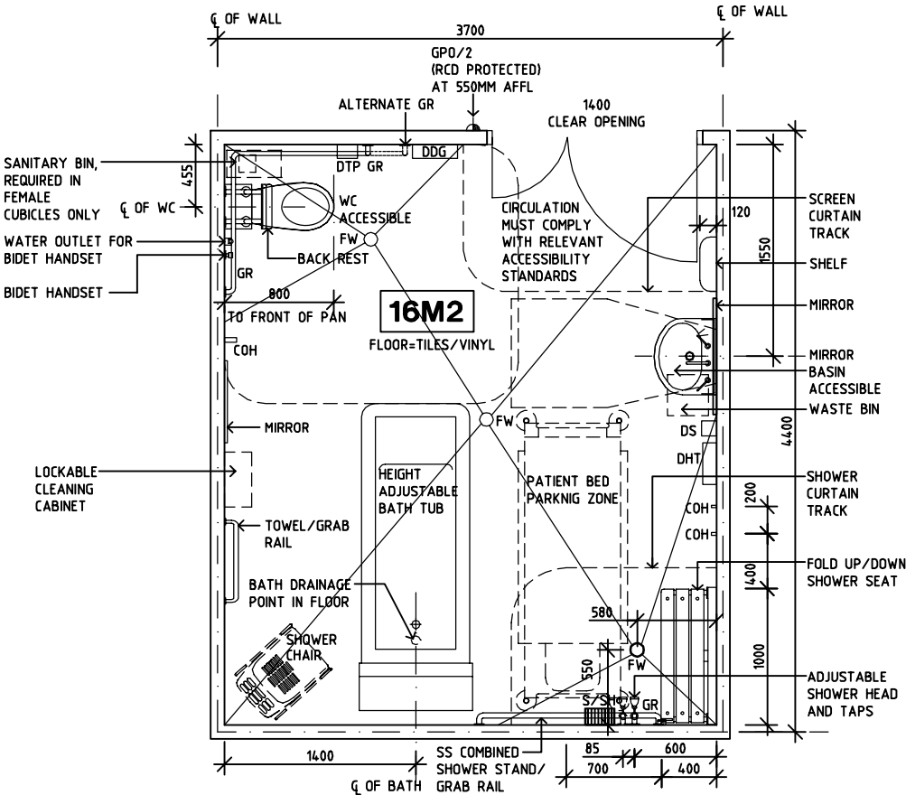
PLAN
