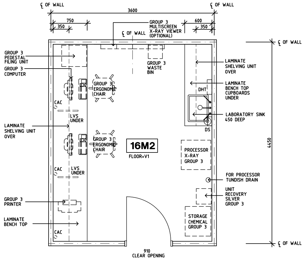
PLAN
