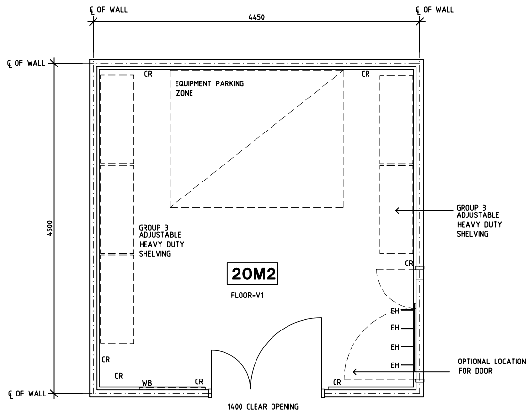
PLAN
