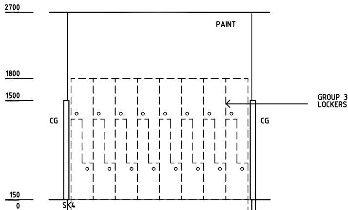
ELEVATION 2 OPTION FOR INTERLOCKED HALF LOCKERS
