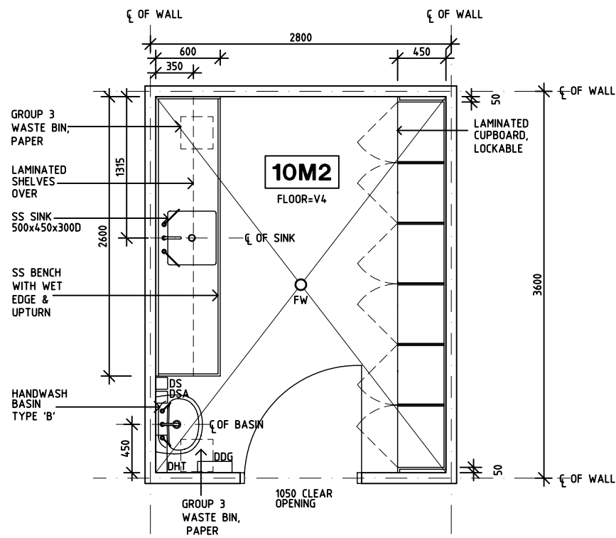
PLAN
