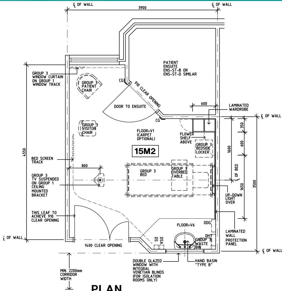
PLAN
