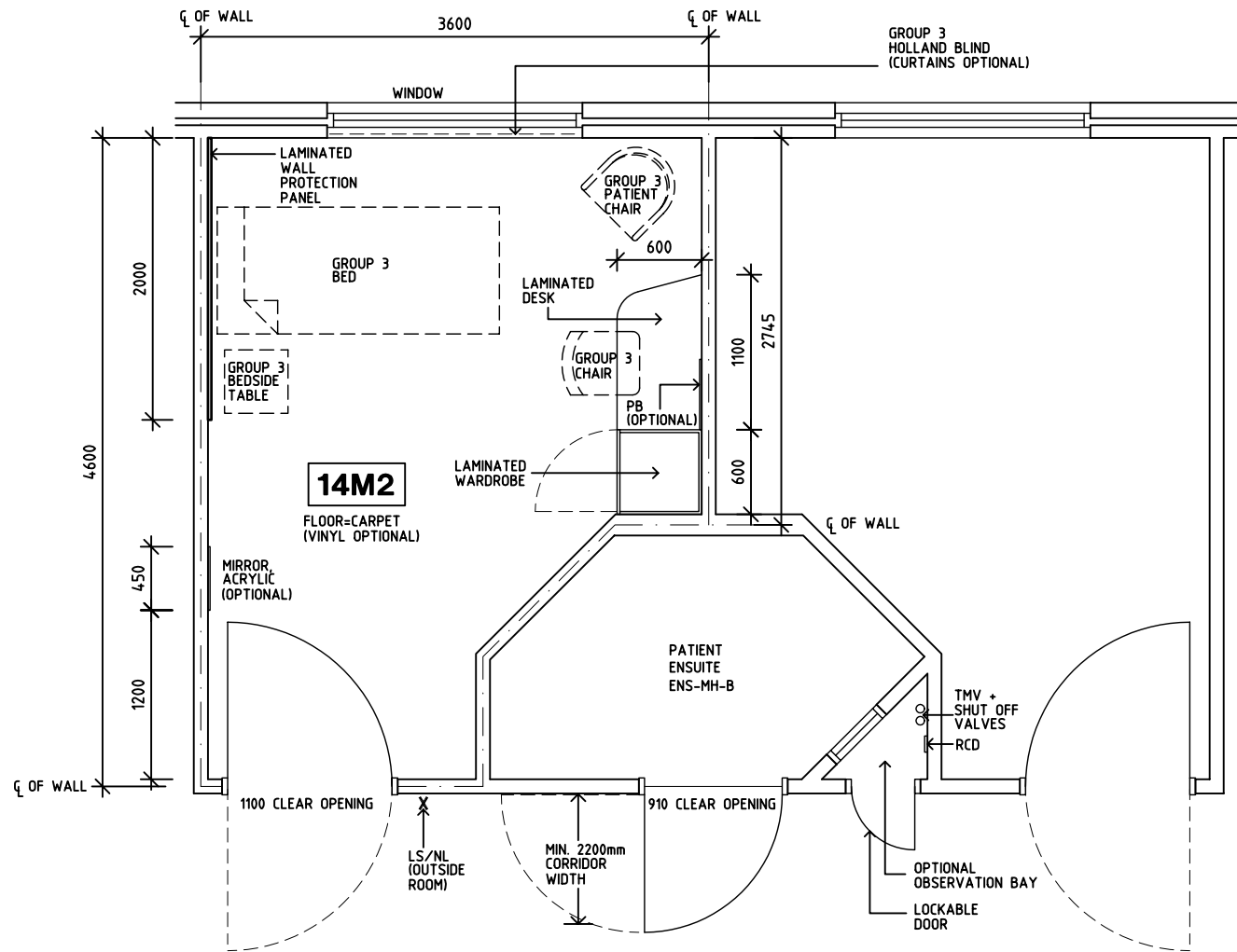
PLAN
