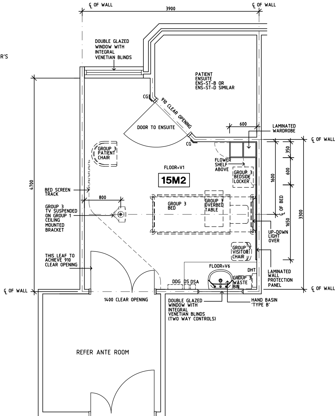
PLAN
